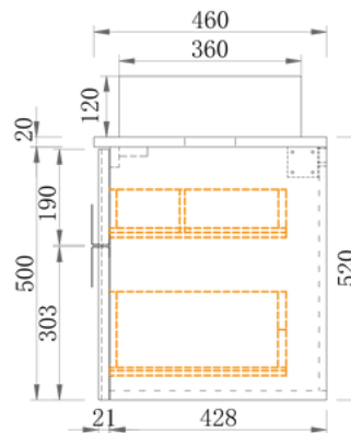
Section Side
